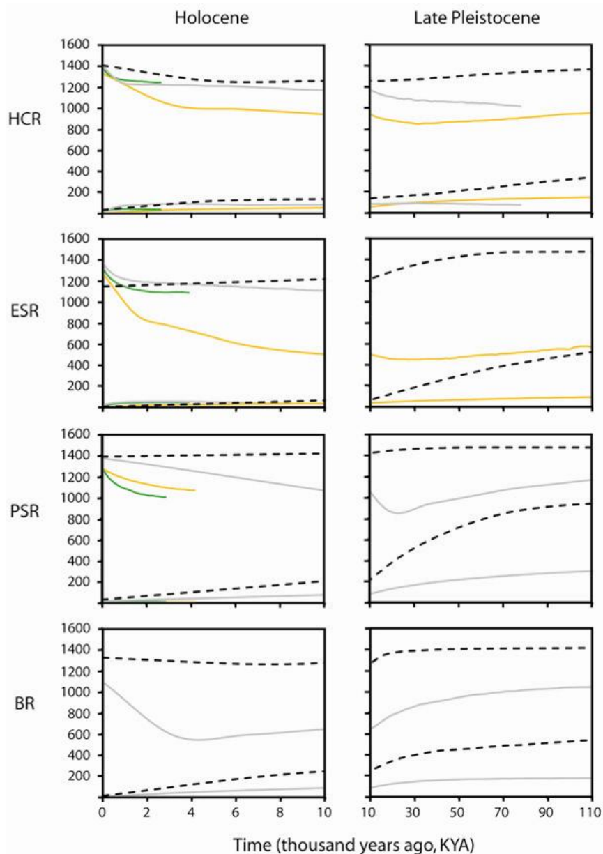
Figure S1. Confidence intervals associated with Bayesian Skyline plots showing changes in N_e over time, based in mtDNA sequence data (Figure 5 of the main text). Curves represent the upper and lower 95% highest posterior density limits for N_e -values (y-axis) plotted over time (x-axis). Curve colours approximate colours of the species themselves (Figure 2 of the main text) and are as follows: Pseudachorutinae sp., pale gray; Acanthanura sp., black (dashed); Artioposthia lucasi , yellow; and Caenoplana coerulea , dark green (note that A. lucasi population PSR corresponds with PSR-1 in Figure 3 of the main text). Note that for a given population, Holocene vs. Late Pleistocene represents the same analysis (rescaled).
